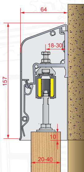
1-channel mounting
