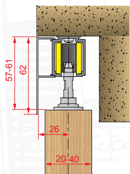
Ceiling mounting
