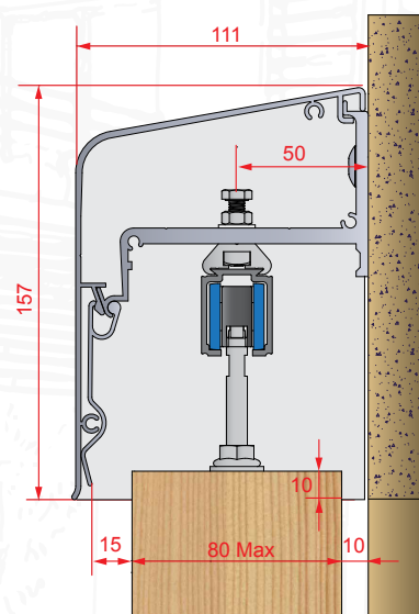
Shade screen mounting (up to 120 kg)
