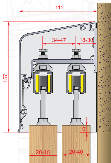
2-channel mounting
